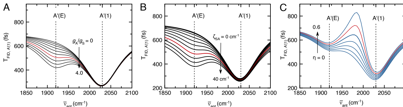
Fig. 5. Model T_{\text{FID},A'(1)} as a function of antenna frequency \bar{\nu}_{\text{ant}} , obtained from 1/T_{\text{FID}}^0 + 1/2T_{1,P} + 1/2T_{1,\text{IVR-P}} . (A) For varying ratios of the oscillator strengths 0 \leq g_A/g_S \leq 4.0 , for fixed vibration–vibration coupling \zeta_{\text{SA}} = 25 \text{ cm}^{-1} , g_S = 20 \text{ cm}^{-1} and weighting anti-Purcell factor \eta = 0 . (B) For varying 0 \leq \zeta_{\text{SA}} < 40 \text{ cm}^{-1} , with fixed ratio g_A/g_S = 3.3 and \eta = 0 . (C) For varying 0 \leq \eta < 0.6 , g_A/g_S = 2.7 and \zeta_{\text{SA}} = 25 \text{ cm}^{-1} . The red marked lines correspond to the parameters with the best fit to the experimental data in Fig. 4A.
