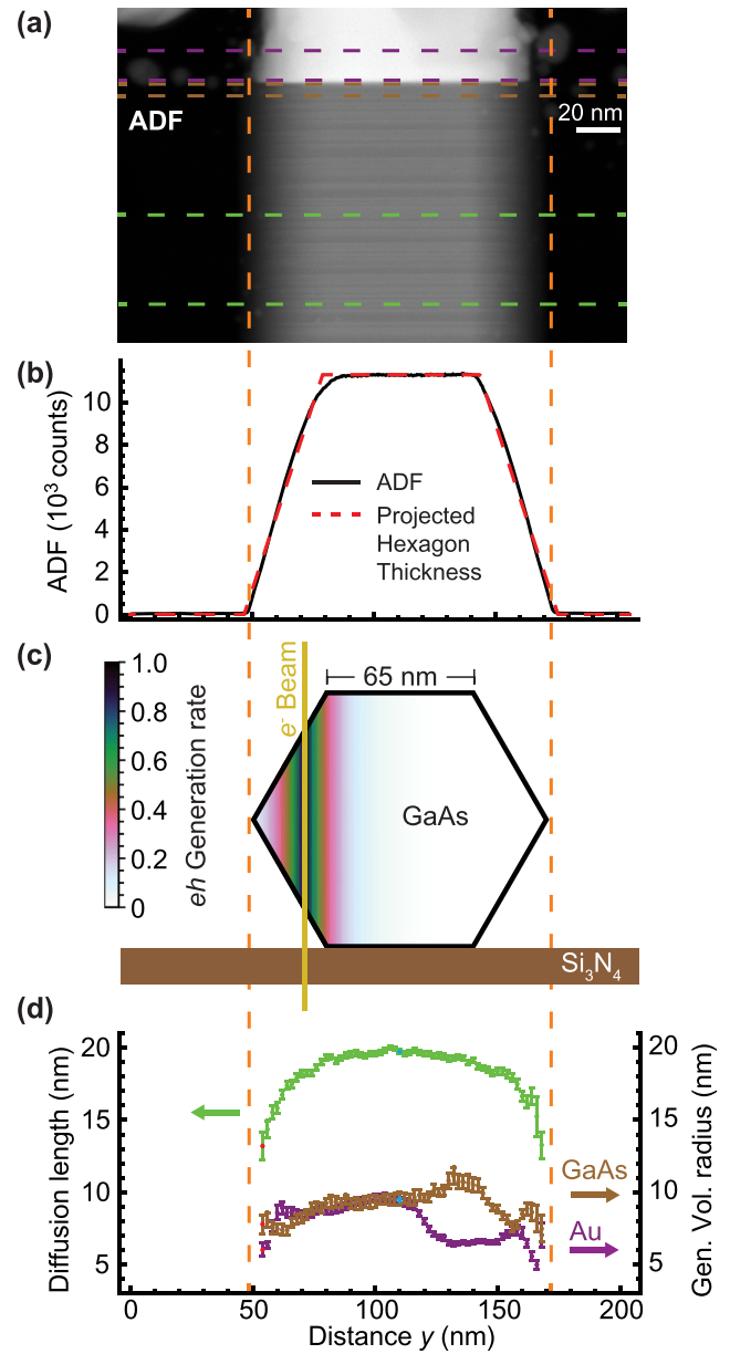
FIG. 3. Mapping eh recombination across the nanowire. (a) The data of Fig. 2(a) are rotated 90° to align the Schottky interface with the horizontal axis. Summing the ADF signal from the dashed green ROI in (a) gives a profile (b) approximately proportional to the sample thickness. This profile agrees well with the projected thickness of a geometrically perfect hexagon [dashed red line in (b)]. A slice of the cylindrical eh -generation volume is overlaid on the nanowire cross section (c), with a decay radius R = 10 nm. The generation volume radii R in Au and GaAs and the minority-carrier diffusion length L in the GaAs are plotted as a function of radial position across the hexagonal nanowire in (d). The L and R measurements shown explicitly in Fig. 2(d) are highlighted in blue (center) and red (edge) here. All panels are aligned horizontally on the same distance axis.
