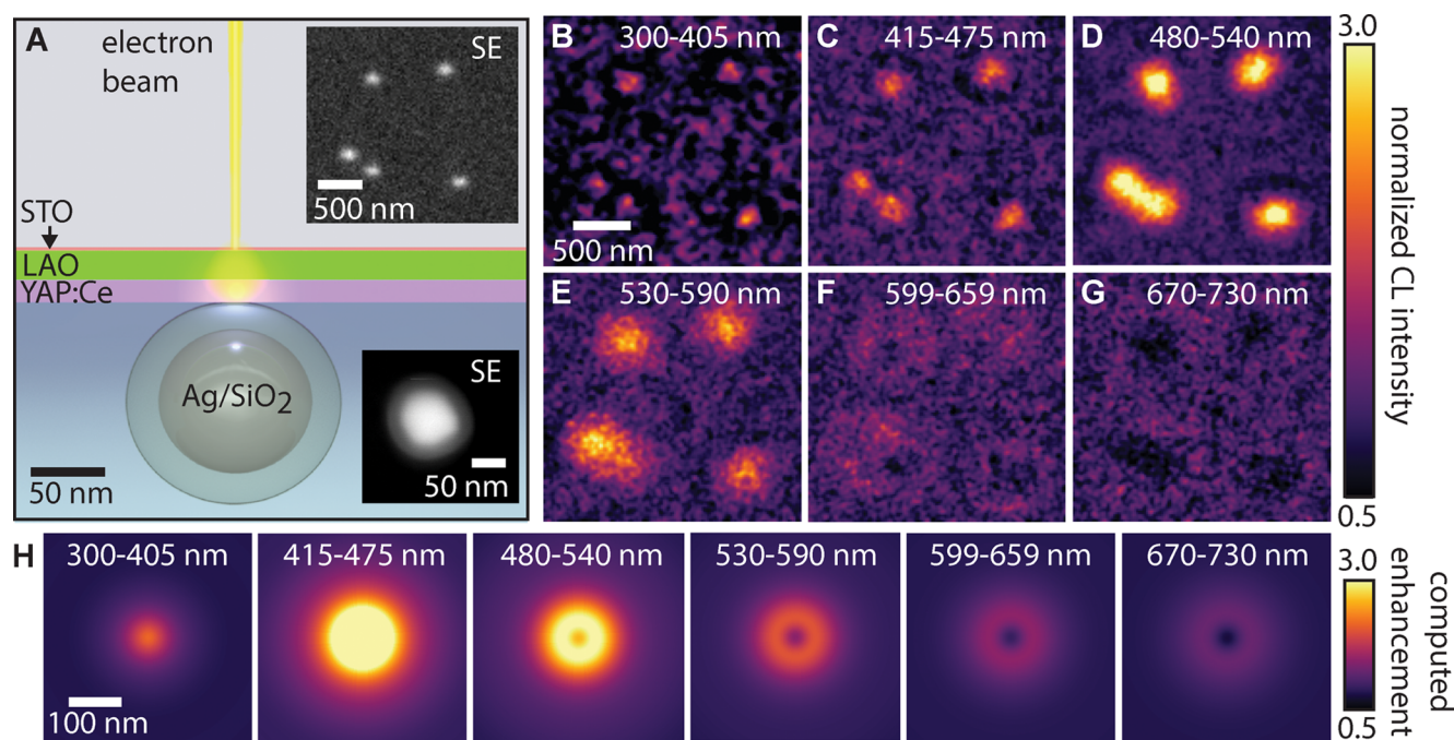
Figure 4. CLAIRE imaging and simulated CLAIRE images of 100 nm Ag particles with a 20 nm SiO 2 shell. (A) Schematic of CLAIRE imaging of 100 nm Ag particles with a 20 nm SiO 2 shell with SEM image of the Ag/SiO 2 core-shell particles through the free-standing YAP:Ce film at 10 kV in the upper inset and SEM image of the Ag/SiO 2 core-shell particles in the lower inset. (B–G) CLAIRE images of the Ag/SiO 2 core-shell nanoparticles acquired with different emission filters. The images are normalized with respect to the background, which is set at 1, and the maximum of all six images. (H) Simulated CLAIRE images of Ag/SiO 2 core-shell nanoparticles at different emission wavelengths.
