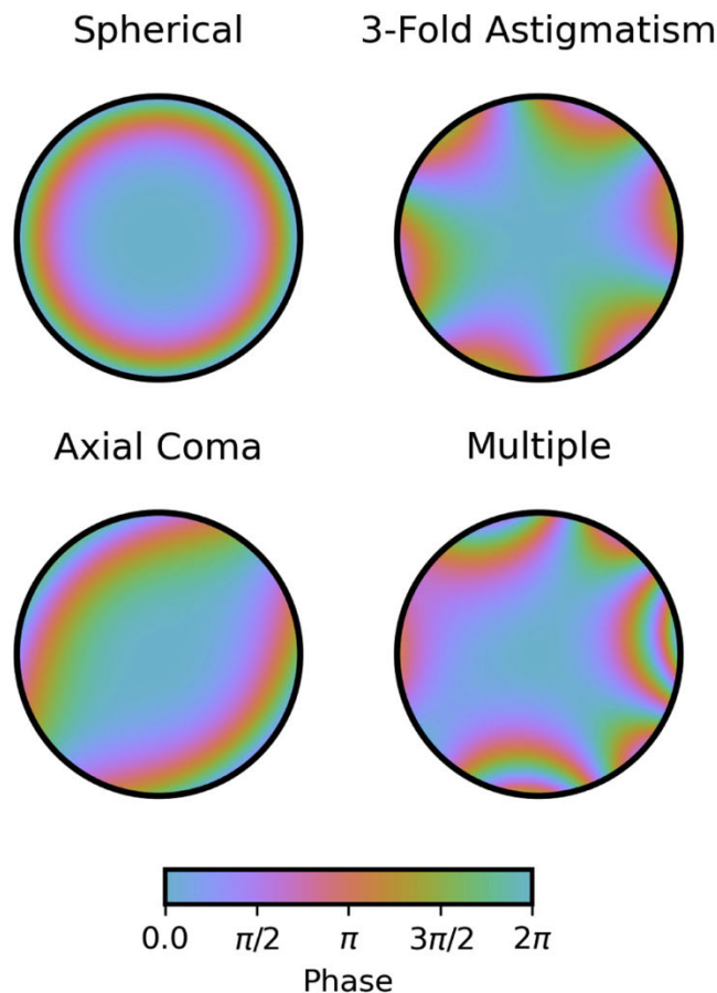
Fig. 4. Example aberration phase plates. From top-left to bottom-right, spherical aberration, 3-fold astigmatism, axial coma, and an arbitrary mixture of aberrations at 300 kV. Borders represent a cutoff of 2 inverse angstroms.
