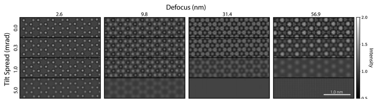
Fig. 12. Simulated HRTEM images of monolayer \text{WS}_2 at 300 kV with limited coherence. Results shown at different contrast maxima (increasing defocus left to right) and different levels of coherence (increasing tilt spread top to bottom). Images at a given tilt spread are incoherently averaged with Gaussian weights over tilted plane waves \pm 3\sigma from the untilted beam. All results are similarly incoherently averaged over a focal spread of 10 Å.
