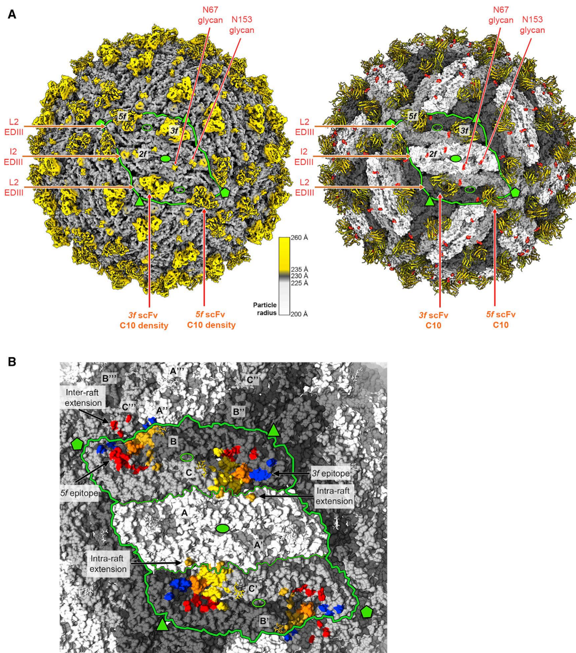
Figure 4. Cryo-EM structure of the DENV2 virion bound to scFv
