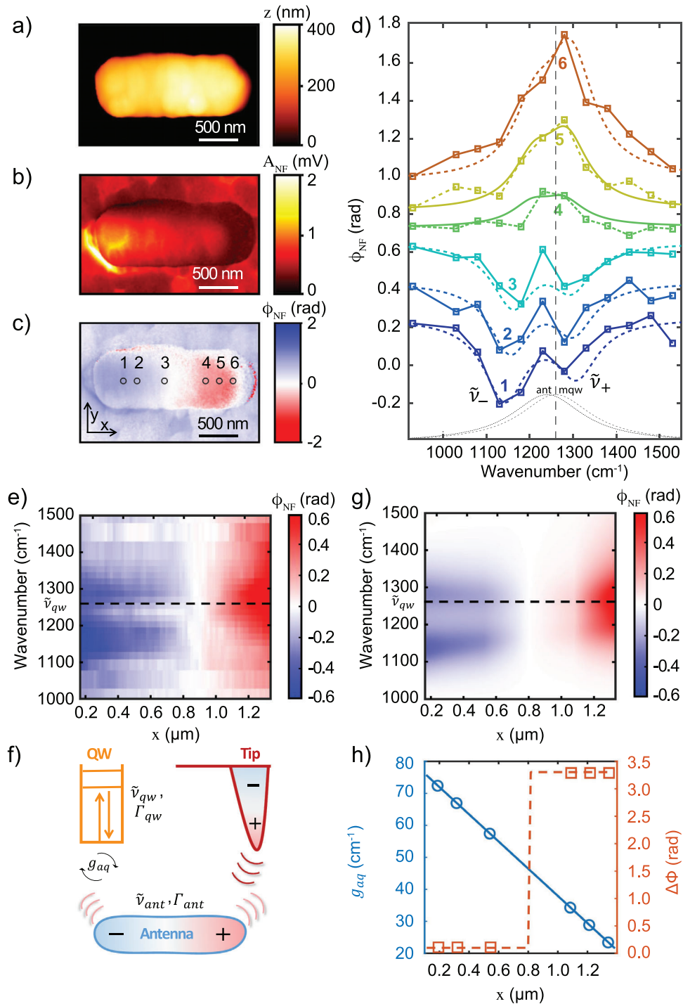
Figure 3. Tip-enhanced control of antenna-MQW strong coupling IR s-SNOM nano-imaging of a single antenna-MQW structure, a) topography, b) amplitude A_{NF} with a laser tuned to 1330\text{ cm}^{-1} , and c) corresponding phase \phi_{NF} . d) Spectra of \phi_{NF} measured as a function of tip positions across the antenna (open circles in c), with MQW ISB transition frequency \tilde{\nu}_{qw} = 1260\text{ cm}^{-1} (black dashed). e) Surface plot of the \phi_{NF} spectra measured as a function of tip position x along the antenna in steps of 15\text{ nm} , with MQW ISB transition frequency \tilde{\nu}_{qw} = 1260\text{ cm}^{-1} (black dashed). f) Schematic of coupling between antenna, MQW, and AFM tip. The non-resonant tip-antenna interaction modifies the local driving field through spatial antenna phase-dependent near-field interference. g) Surface plot of modeled \phi_{NF} spectra as a function of tip position x for the \Delta\phi and g_{aq} parameters shown in (h). h) Modeled coupling strength g_{aq} and \Delta\phi as a function of tip position x along the antenna length.
