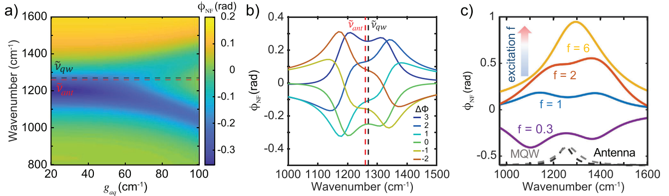
Figure 4. Classical and quantum model of antenna-MQW strong coupling a) Spectral evolution based on coupled-oscillator modeling as a function of g_{aq} , with the asymmetric splitting of the two polaritonic states, with \Delta\phi = 0.5 rad, \tilde{\nu}_{ant} = 1240 \text{cm}^{-1} and \tilde{\nu}_{qw} = 1260 \text{cm}^{-1} . b) Spectra with g_{aq} = 75 \text{cm}^{-1} , varying the \Delta\phi from 3 to -2 rad. c) The spectra of \phi_{NF} based on density matrix formalism for four different excitation field amplitudes f and phases.
