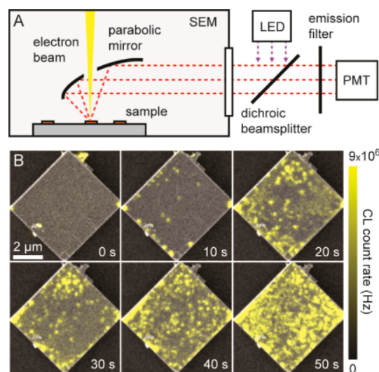
Figure 2. High-resolution cathodoluminescence (CL) imaging of photoinduced phase separation in a single nanoplate. (A) CL detection apparatus. (B) Sequence of CL images with a 650 nm long pass filter interleaved by 10 s of illumination at 405 nm (100 \text{mW}/\text{cm}^2 ) between each frame.
